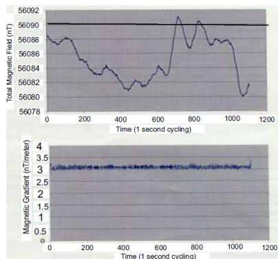
Sample data Gradiometer data shows very low noise level (<0.2nT. peak to peak)
